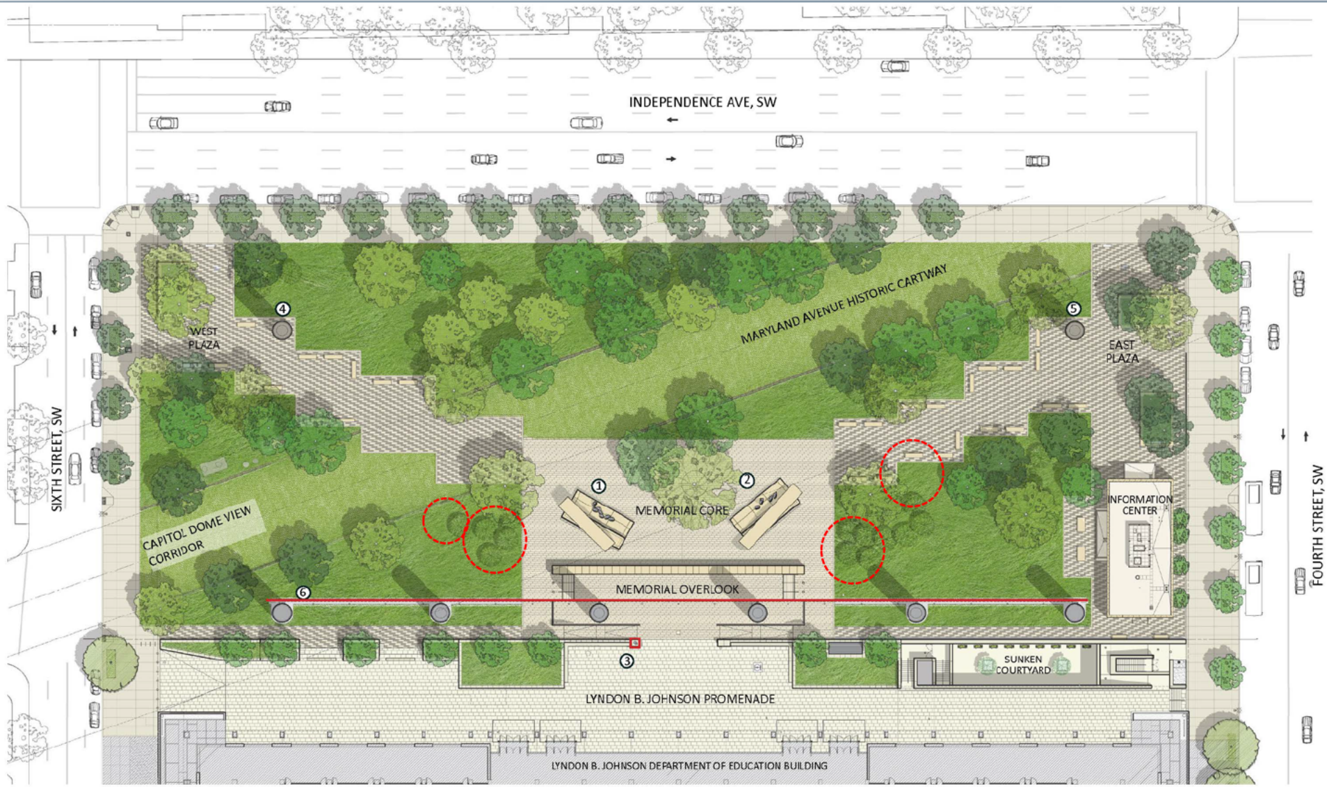
0' 5' 10' 25' 50' SITE PLAN
